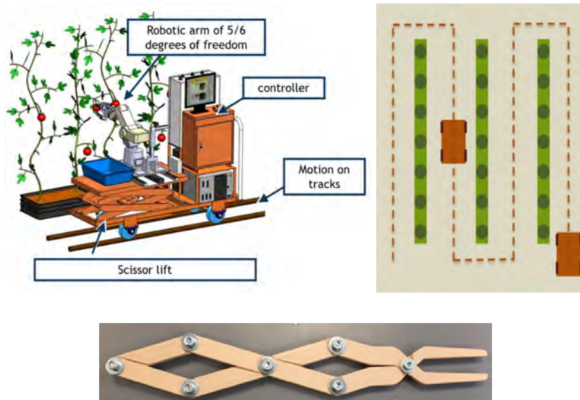
Fig. 3. The design of the robotic platform, its motion on tracks in the greenhouse and the robotic end-effector.
